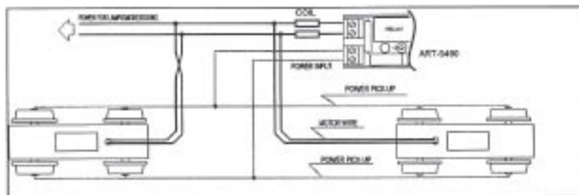
TYPICAL WIRING DIAGRAM FOR OTHER LOCOMOTIVES
