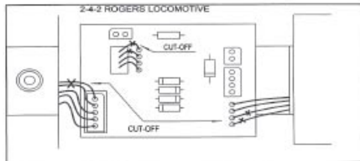
(2-4-2 ROGERS LOCOMOTIVE)
